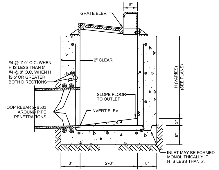
WR CURB INLET (SINGLE)
