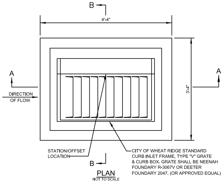
WR CURB INLET (SINGLE)
