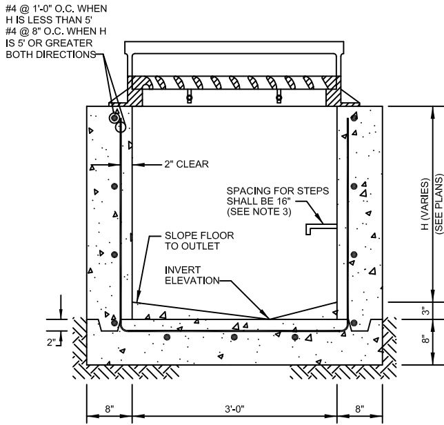
WR CURB INLET (SINGLE)
