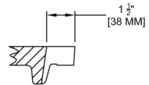
PICKHOLE DETAIL
